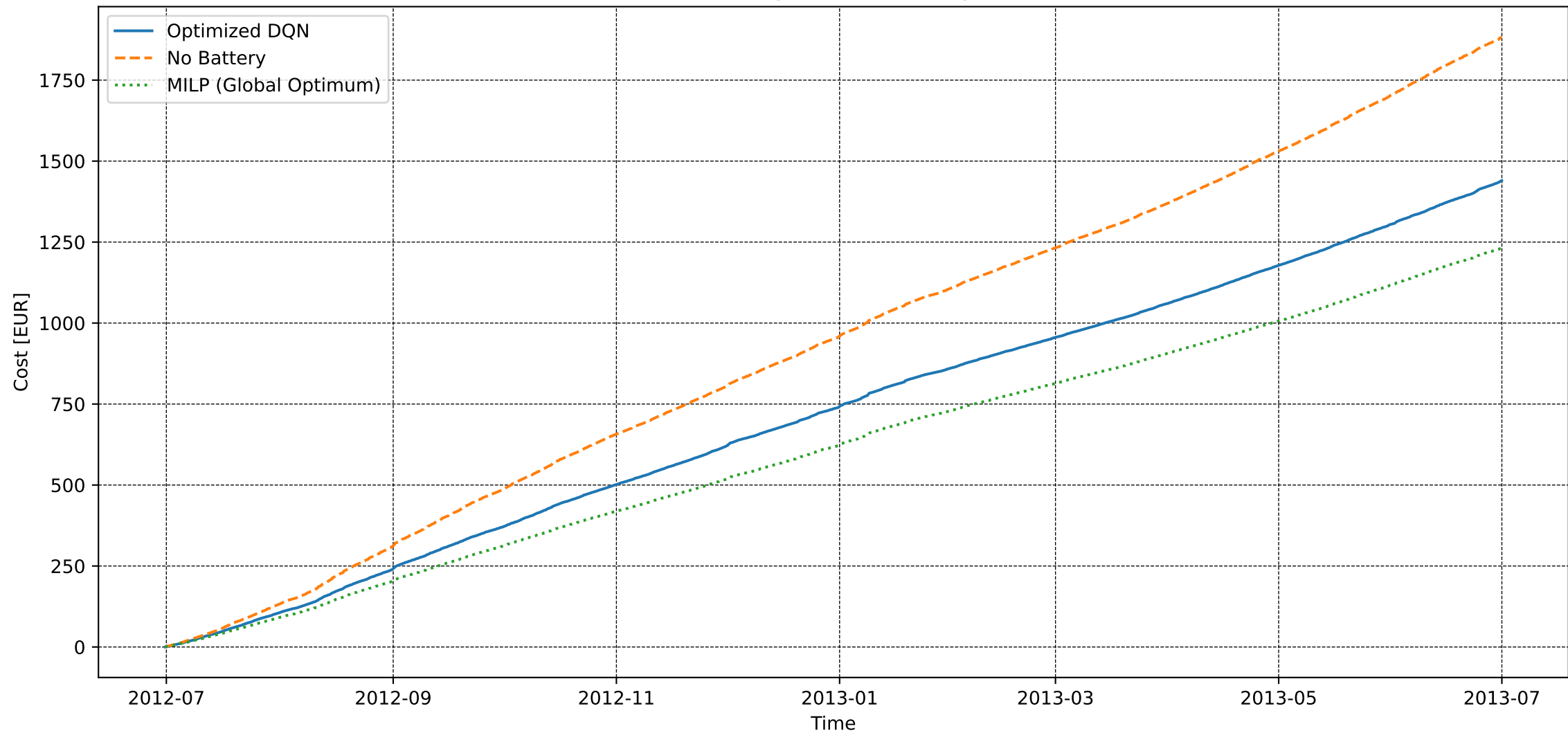
User 21 - Extended Convergence - Electricity Cost [DQN vs MILP]
